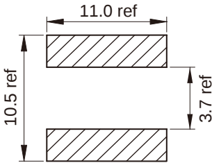
Land Pattern: [mm]
